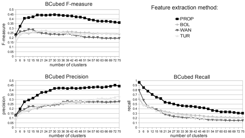
Figure 2: Clustering quality in terms of precision, recall and F_1 -measure on the R30 dataset. The proposed feature generation approach (black line, square data points) outperforms all baseline approaches.
